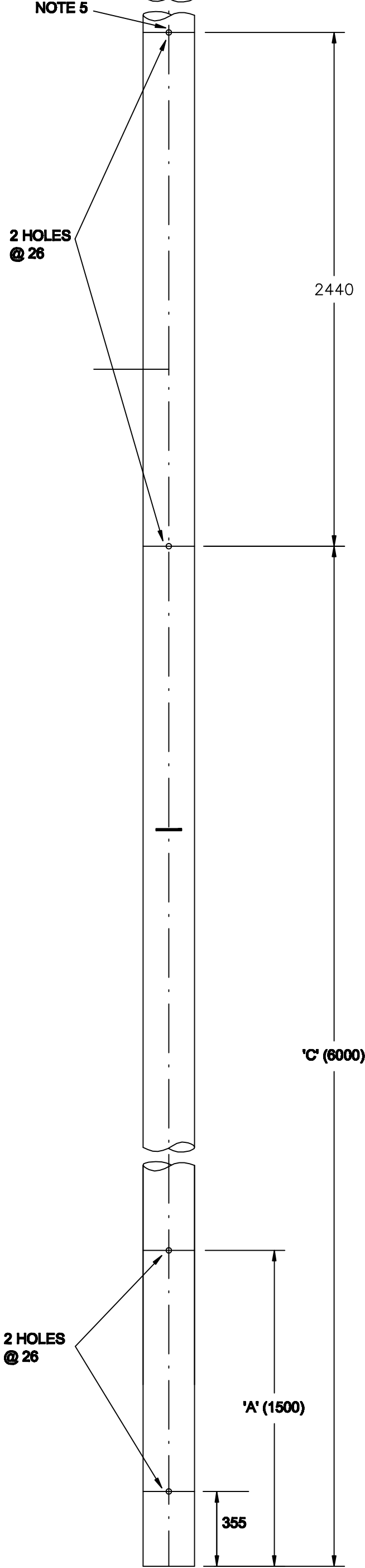
SLACK SPAN 'H' TERMINAL SUPPORT (TYPE 3)
